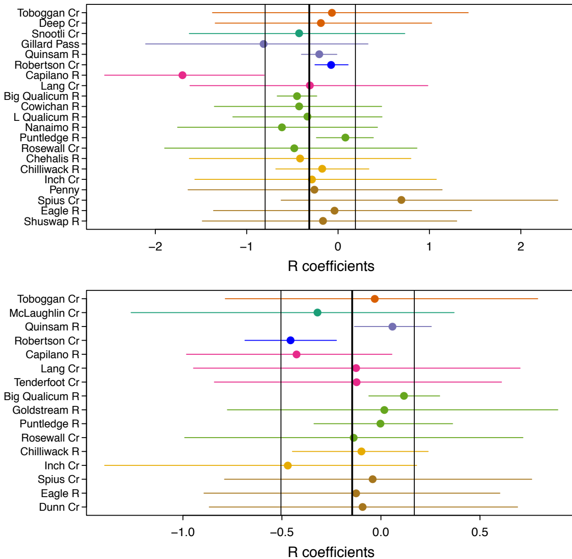
Figure 8. Multi-hatchery Chinook (top) and Coho (bottom) survival model coefficient estimates for the release biomass ( R ) predictor. The circles indicate hatchery specific mean posterior estimates along with 95% credible intervals, while the vertical lines indicate the mean posterior for the average effect across all hatcheries (thick black line) with 95% credible intervals for the posterior distribution (thin black lines). Colours represent the different production areas (SKNA = Skeena, CC = Central Coast, JNST = Johnstone Strait, SWVI = Southwest Vancouver Island, GSMN = Georgia Strait mainland side, GSVI = Georgia Strait Vancouver Island side, LWFR = lower Fraser River, UPFR/TOMM = upper Fraser River and Thompson River). Source: Part III report, Doherty and Cox 2021.
