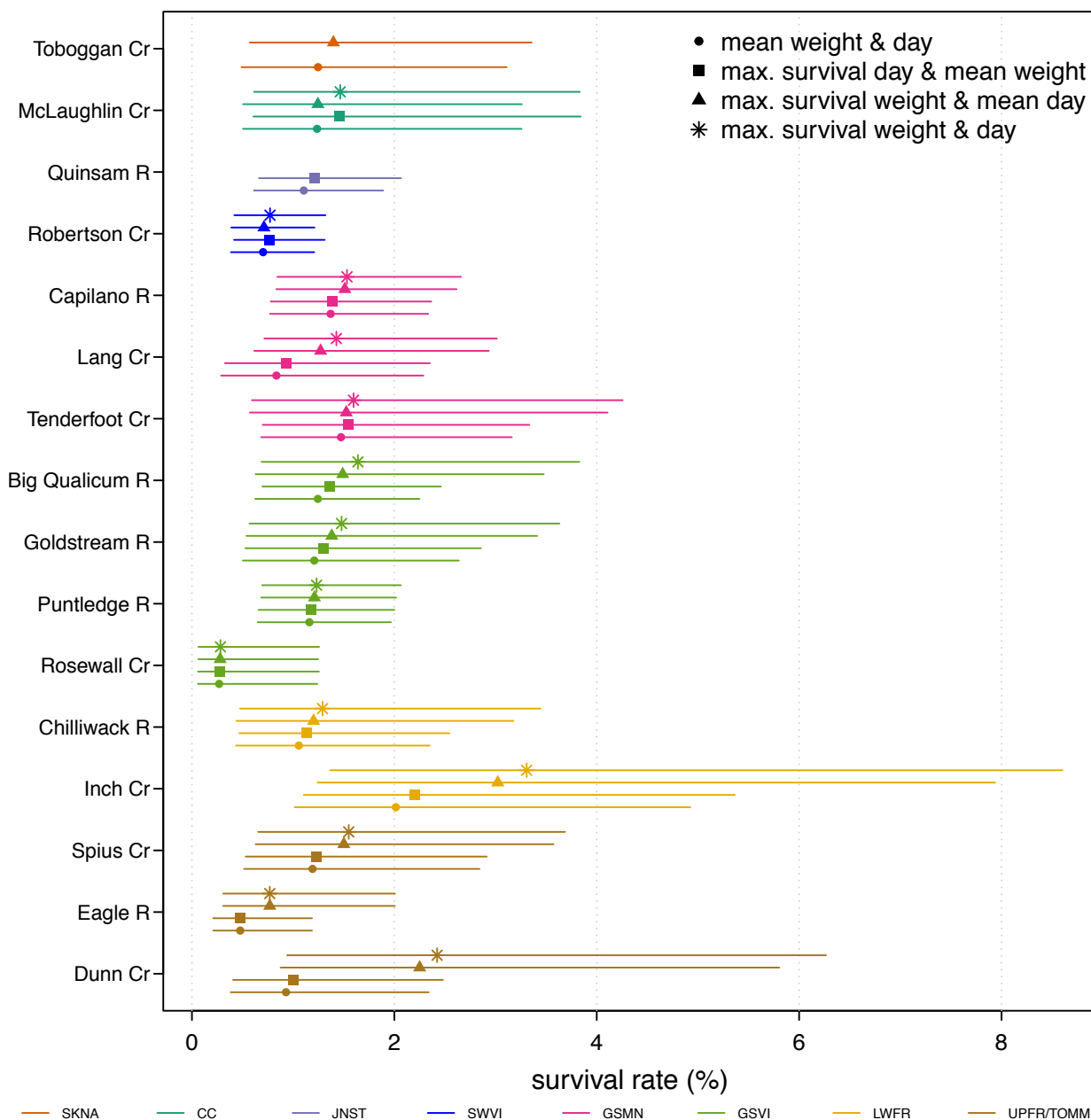
Figure 5. Predicted Coho smolt-to-adult survival rates for 2000-2017 ocean entry years for different release weights and days relative to the mean release weight and day. For each hatchery, the survival rates are estimated for release weights and/or days within the historical observations that are expected to maximize survival for the life stage most commonly released. Points indicate median posterior estimates, while error bars show 95% credible intervals. Values shown are for fry releases at Eagle River and Rosewall Creek, and yearling smolts for all other hatcheries. Colours represent the different production areas (SKNA = Skeena, CC = Central Coast, JNST = Johnstone Strait, SWVI = Southwest Vancouver Island, GSMN = Georgia Strait mainland side, GSVI = Georgia Strait Vancouver Island side, LWFR = lower Fraser River, UPFR/TOMM = upper Fraser River and Thompson River). Source: Part III report, Doherty and Cox 2021.
