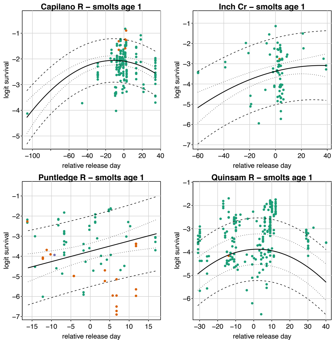
Figure A.8. Mean logit survival (solid line) for Coho at release days for hatchery and life-stage specific model fits. The 95% CIs are shown for fixed effects only (dotted lines) and for both fixed and random year effects (dashed lines). The zero day indicates the mean release date for a hatchery and different colours indicate different stocks.
