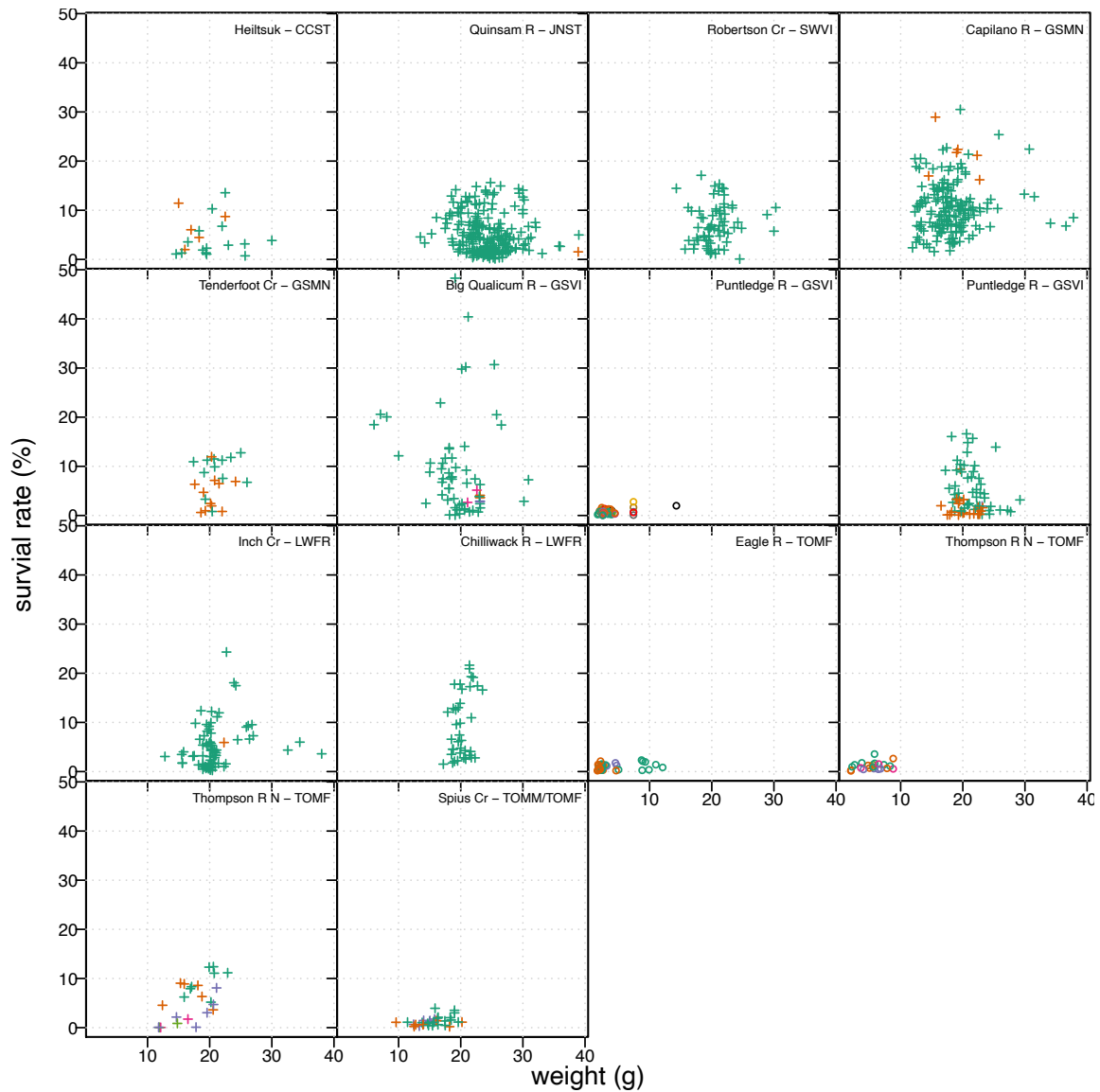
Figure CO.3. Smolt-to-adult survival rates (%) by weight-at-release for fry (O) and yearling (+) CWT Coho hatchery releases included in survival model fitting . Different colors indicate different combinations of stock and release sites for each hatchery with green indicating the most frequent stock released and release site.
