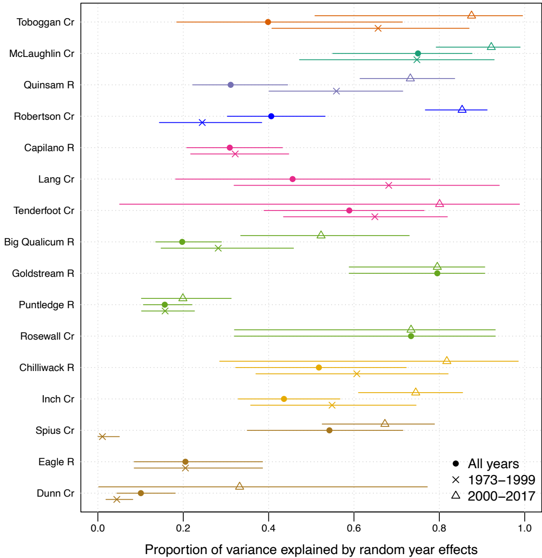
Fig E.6. Proportion of variance ( \rho_h ) in average Coho annual logit-survival rates that is explained by the random year effects for different periods of ocean entry years. The mean posterior \rho_h with 95% credible intervals is shown for each hatchery and time period.
