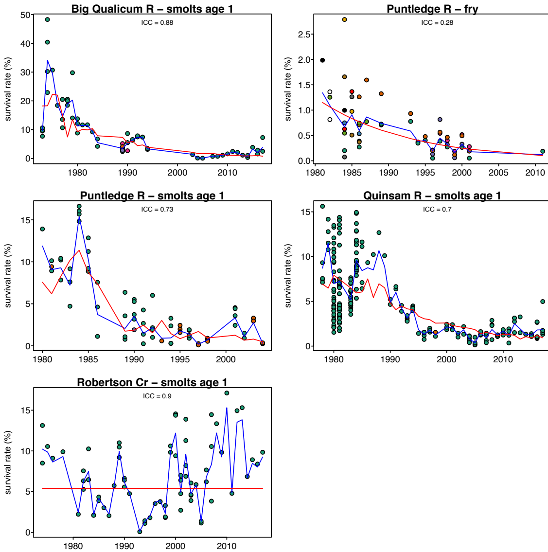
Figure CO.20. Top model fits for Vancouver Island hatcheries' average Coho survival over time, accounting for all predictors (e.g. weight, day, year, stock, and release site) with (blue) and without (red) random year effects. Different colors indicate different combinations of stocks and release sites for each hatchery with green indicating the most frequent stock released and release site.
