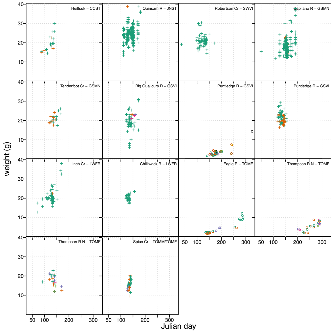
Figure CO.6. Weight-at-release by Julian day for fry (○) and yearling (+) CWT Coho hatchery releases included in survival model fitting . Different colors indicate different combinations of stock and release sites for each hatchery with green indicating the most frequent stock released and release site.
