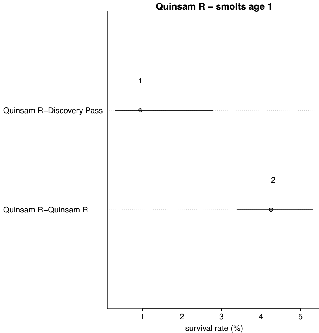
Figure CO.18. Estimated marginal mean Coho survival rates for Quinsam River Hatchery yearling releases at Quinsam River and Discovery Pass seapen. Quinsam River hatchery was the only the Coho survival model that included a release site effect in the top model. The numbers indicate groups whose survival rates are significantly different from one another (i.e., group 1 is different from group 2, but there is no difference between group 12 and 1 or group 12 and 2). Error bars are shown for 95% confidence intervals. The y-axis shows the stock released (Quinsam River) followed by a dash and the release site. Release site locations are shown in Appendix B.
