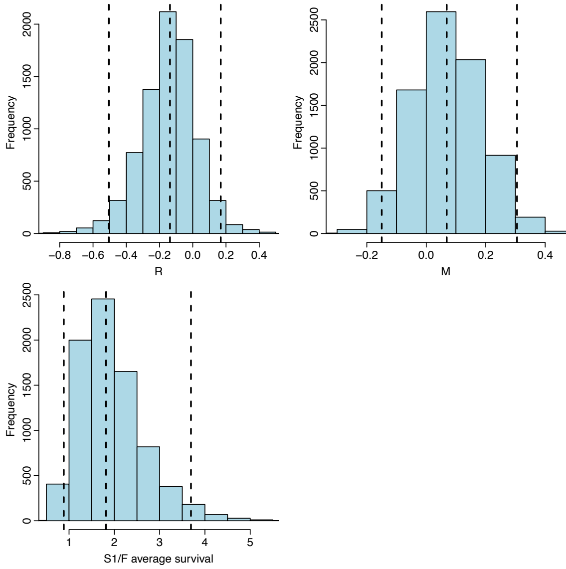
Figure CO.34. Posterior distribution of coefficient estimates for Coho multi-hatchery survival models for hatchery release biomass ( R ), log river migration distance ( M ), and the ratio of yearling smolt to fry (S1/F) survival. For each distribution the vertical dotted lines indicate the 2.5 th , 50 th , and 97.5 th percentiles.
