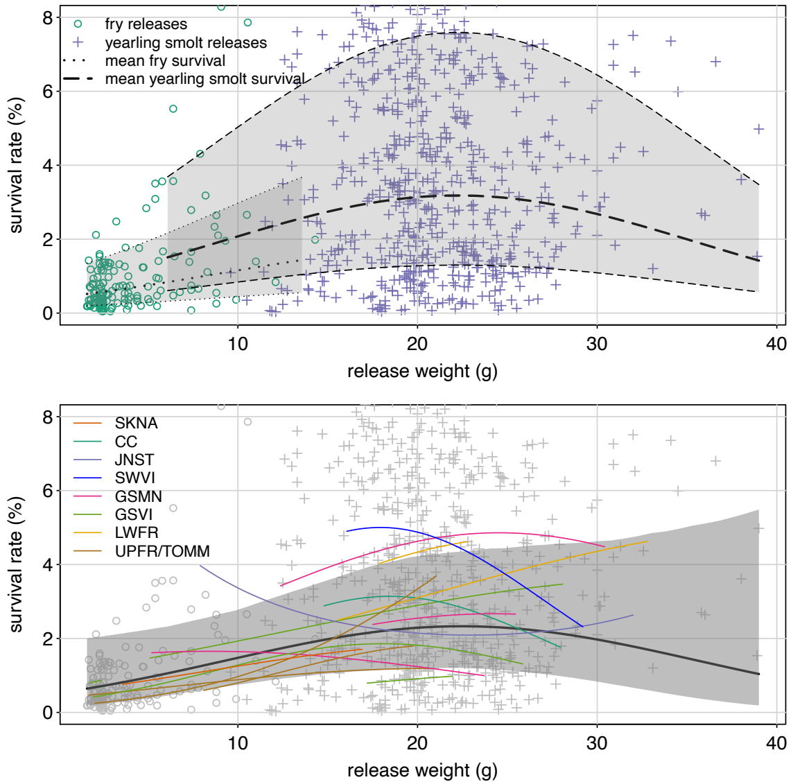
Figure CO.31. Top: Multi-hatchery model fit (MLE) with 95% CIs for average hatchery survival for Coho at different release weights for fry and yearling smolts. Bottom: Hatchery average and hatchery-specific survival responses for the central 95% distribution of observed weights-at-release for each hatchery. The black line (mean posterior) and shaded areas (95% credible interval) indicate the average weight effect on survival across all hatcheries, while coloured lines show hatchery-specific estimates (MLE). Note observations with survival rates greater than 8% are not shown.
