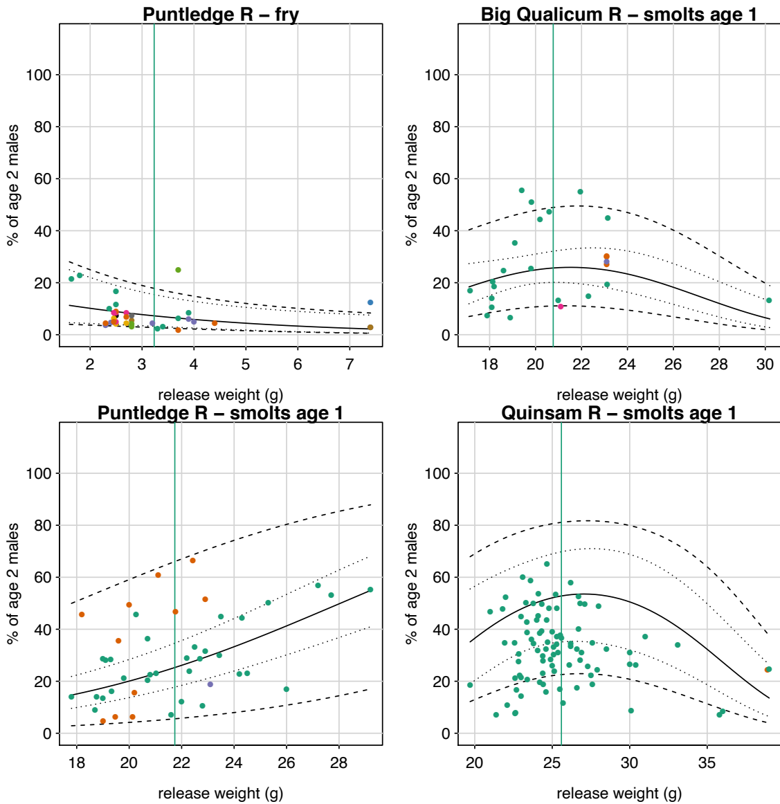
Figure CO.24. Mean % of age-2 male returns (solid line) for Coho at different release weights for hatchery and life-stage specific model fits. The 95% CIs are shown for fixed effects only (dotted lines) and for both fixed and random year effects (dashed lines). Different colours indicate different combinations of stocks and release sites for each hatchery, while the solid green vertical line indicates the mean weight-at-release. Hatcheries without Weight effects in top models are not shown.
