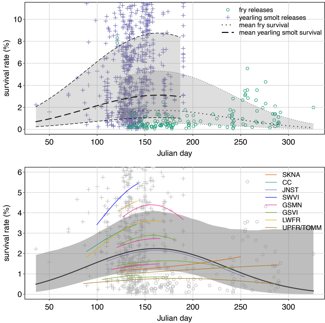
Figure CO.32. Top: Multi-hatchery model fits (MLEs) with 95% CIs for average hatchery survival for Coho at different release days for fry and yearling smolts. Bottom: Hatchery average and hatchery-specific survival responses for the central 95% distribution of observed days-at-release for each hatchery. The black line (mean posterior) and shaded areas (95% credible interval) indicate the average day effect on survival across all hatcheries, while coloured lines show hatchery-specific estimates (MLEs). Note observations with survival rates greater than 10% (top panel) and 6% (bottom panel) are not shown.
