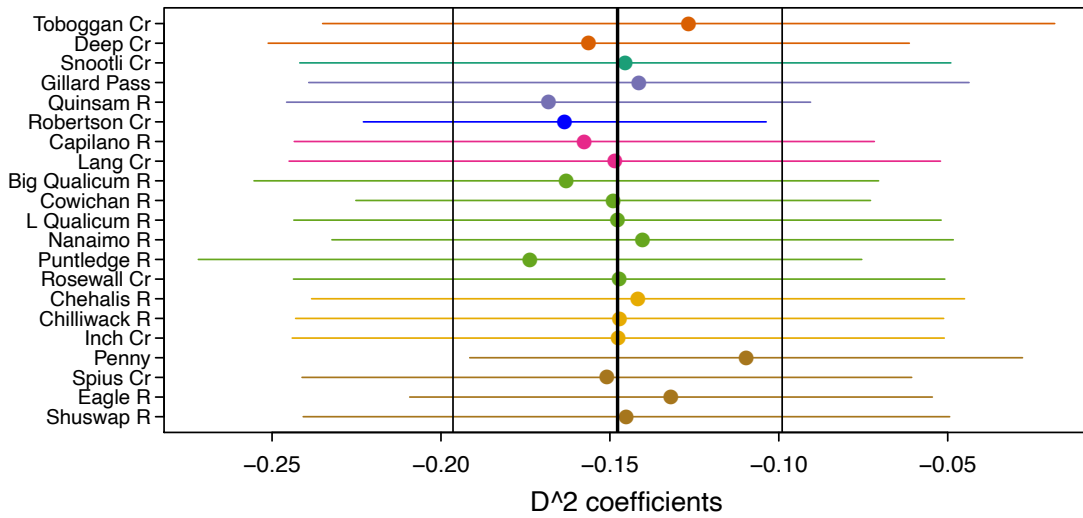
Figure A.14. Multi-hatchery Chinook survival model coefficient estimates for initial model fits including hatchery deviations for quadratic terms for Weight ( W^2 ) and Day ( D^2 ) at-release. The circles indicate hatchery specific estimates along with 95% CIs, while the vertical lines indicate the average effect (thick black line) across all hatcheries with 95% CIs (thin black lines).
