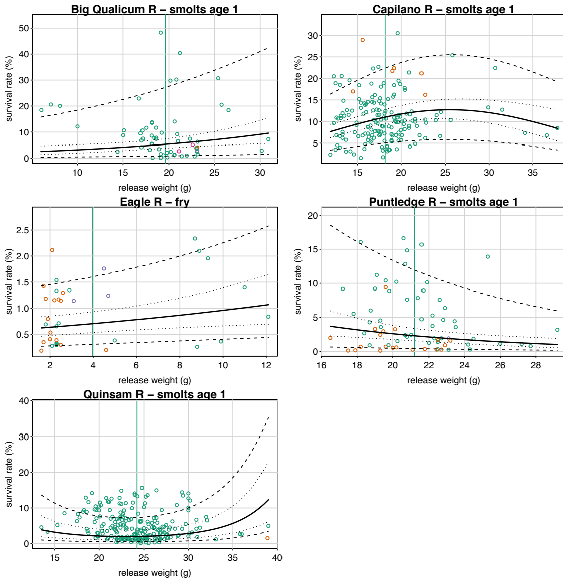
Figure CO.16. Mean survival (solid line) for Coho at different release weights for hatchery and life-stage specific model fits. The 95% CIs are shown for fixed effects only (dotted lines) and for both fixed and random year effects (dashed lines). Different colours indicate different combinations of stocks and release sites for each hatchery, while the solid green vertical line indicates the mean weight-at-release. Hatcheries without Weight effects in top models are not shown.
