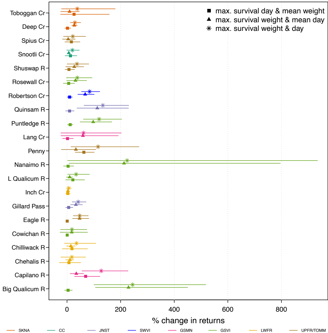
Figure CH.39. Estimated increase in average Chinook returns (%) for 2000-2015 ocean entry years for different release weights and days relative to the mean release weight and day. For each hatchery, the % change in returns is shown for release weights and/or days within the historical observations that are expected to maximize survival for the life-stage most commonly released. Points indicate median posterior estimates, while error bars show 95% credible intervals. Values shown are for fry (Deep Cr), yearling smolts (Penny Creek, Spius Cr, Toboggan Cr) and sub-yearling smolts (all others).
