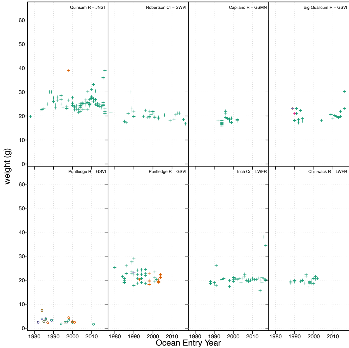
Figure CO.13. Weight-at-release by ocean entry year for fry (○) and yearling (+) CWT Coho hatchery releases included in return age model fitting . Different colors indicate different combinations of stock and release sites for each hatchery with green indicating the most frequent stock released and release site.
