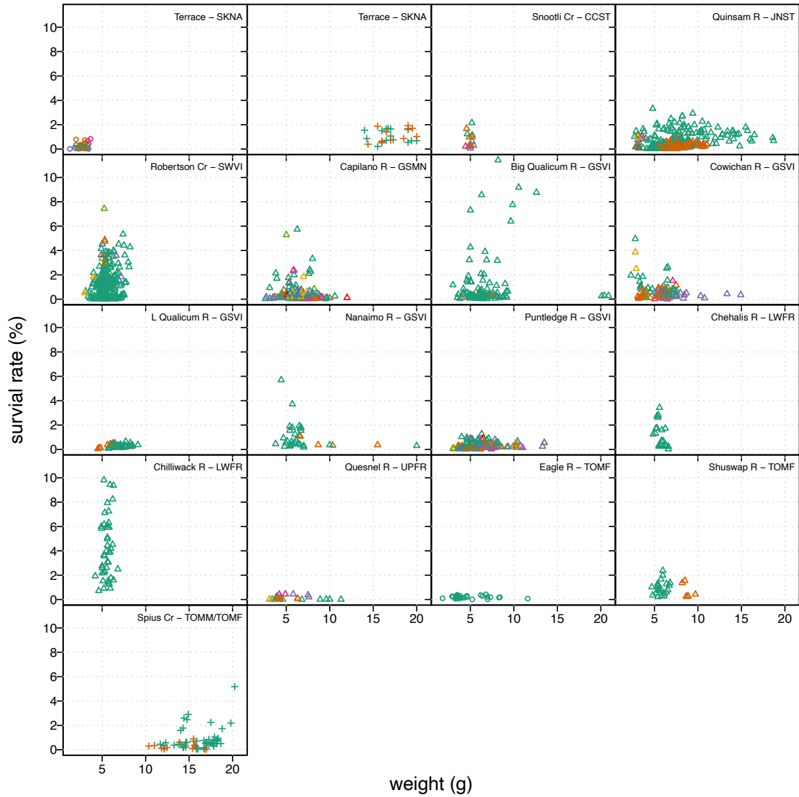
Figure CH.3. Smolt-to-adult survival rates (%) by weight-at-release for fry (○), smolt (△), and yearling (+) CWT Chinook hatchery releases included in survival model fitting . Different colors indicate different combinations of stock and release sites for each hatchery with green indicating the most frequent stock released and release site.
