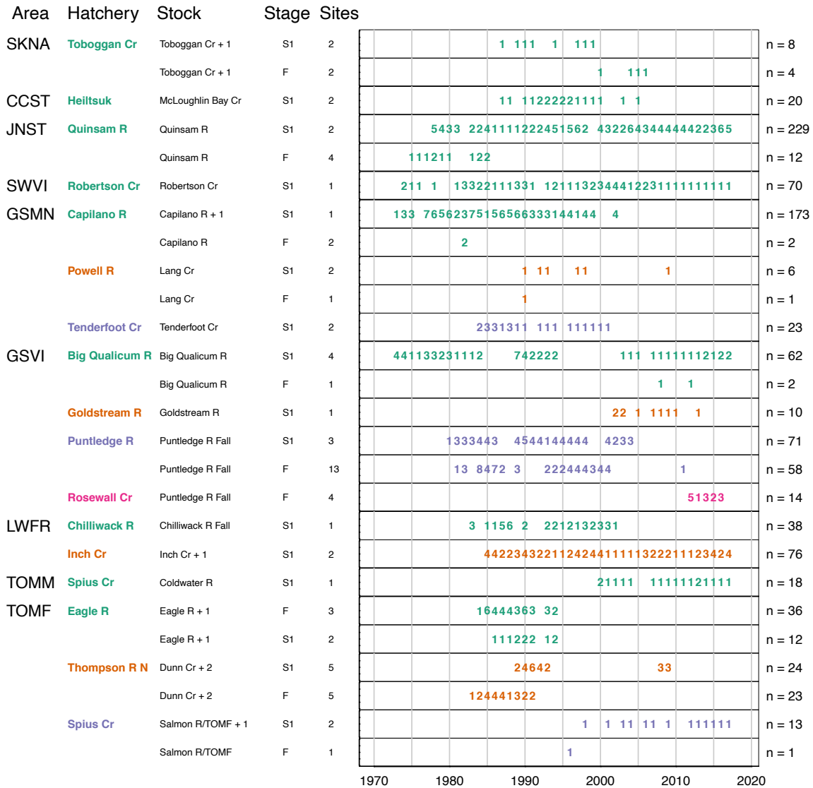
Figure CO.28: Coho CWT fry (F) and yearling smolt (S1) releases by ocean entry year used for fitting multi-hatchery survival models with multiple life-stages. Releases are grouped by hatchery and release site sub-areas (CCST=Central Coast, RIVR=Rivers inlet, SKNA = Skeena River, JNST= Johnstone Strait, SWVI=Southwest Vancouver Island, GSMN = Strait of Georgia Mainland, GSVI = Strait of Georgia Vancouver Island, UPFR = Upper Fraser, LWFR = Lower Fraser, TOMM= Lower Thompson, TOMF= Upper Thompson). Different colours are used to distinguish different hatchery releases in each sub-area.
