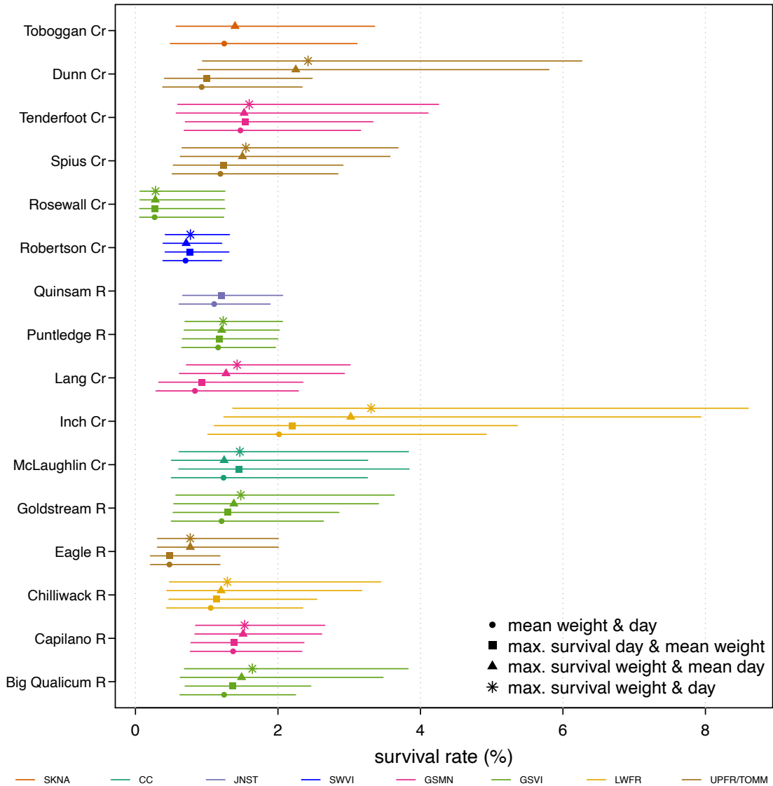
Figure D.3. Predicted Coho smolt-to-adult survival rates for 2000-2017 ocean entry years for different release weights and days relative to the mean release weight and day (●). For each hatchery, the survival rates are estimated for release weights and/or days within the historical observations that are expected to maximize survival for the life-stage most commonly released. Points indicate median posterior estimates, while error bars show 95% credible intervals. Values shown are for fry releases at Eagle River and Rosewall Creek, and yearling smolts for all other hatcheries.
