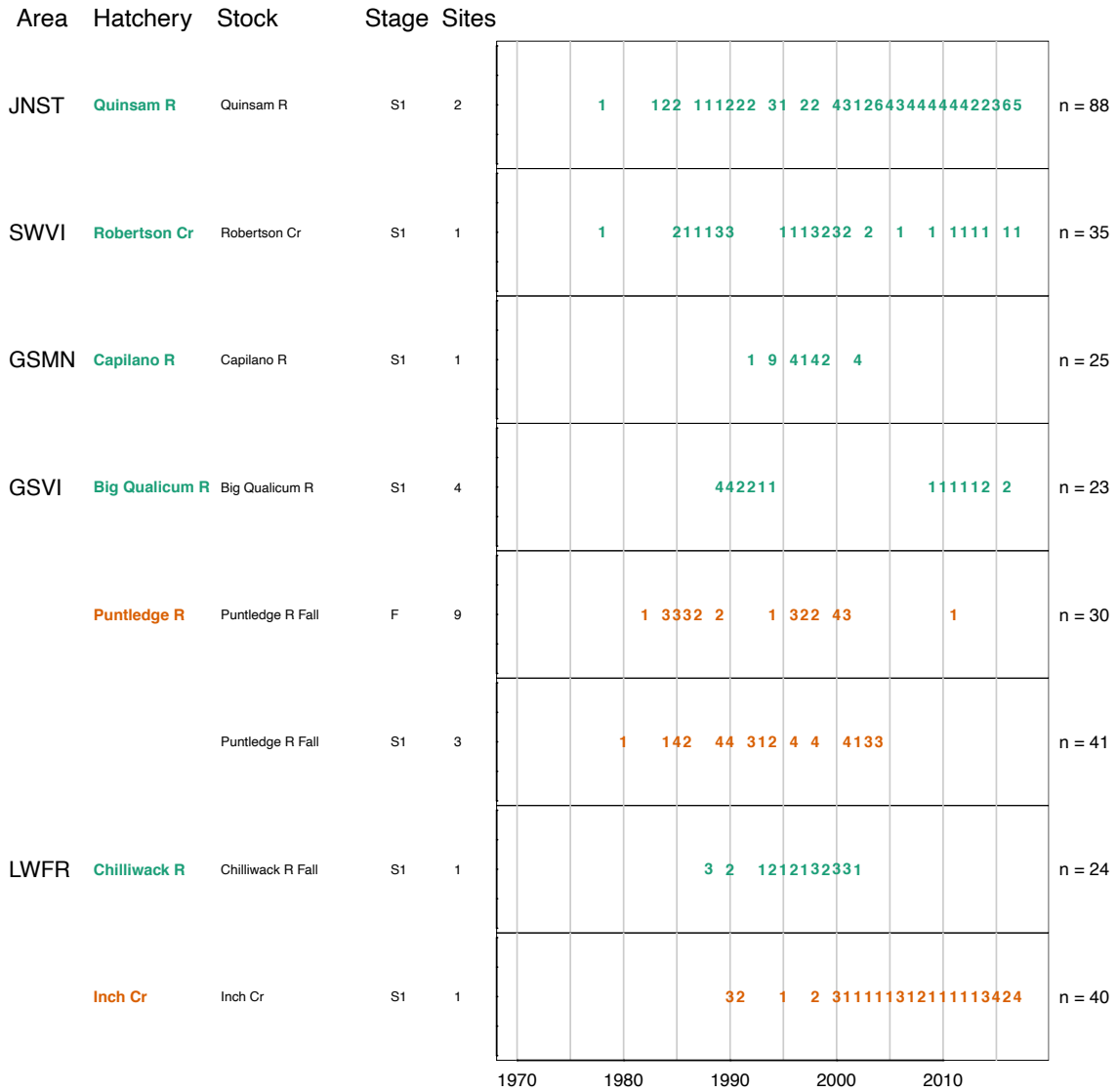
Figure CO.2: Coho CWT hatchery fry (F) and yearling (S1) releases by ocean entry year used for fitting individual hatchery return age models . Releases are grouped by hatchery and release site sub-areas (JNST= Johnstone Strait, GSMN = Strait of Georgia Mainland, GSVI = Strait of Georgia Vancouver Island, LWFR = Lower Fraser, TOMF= Lower Thompson, TOMM= Upper Thompson, SWVI=Southwest Vancouver Island). Different colours are used to distinguish different hatchery releases in each sub-area.
