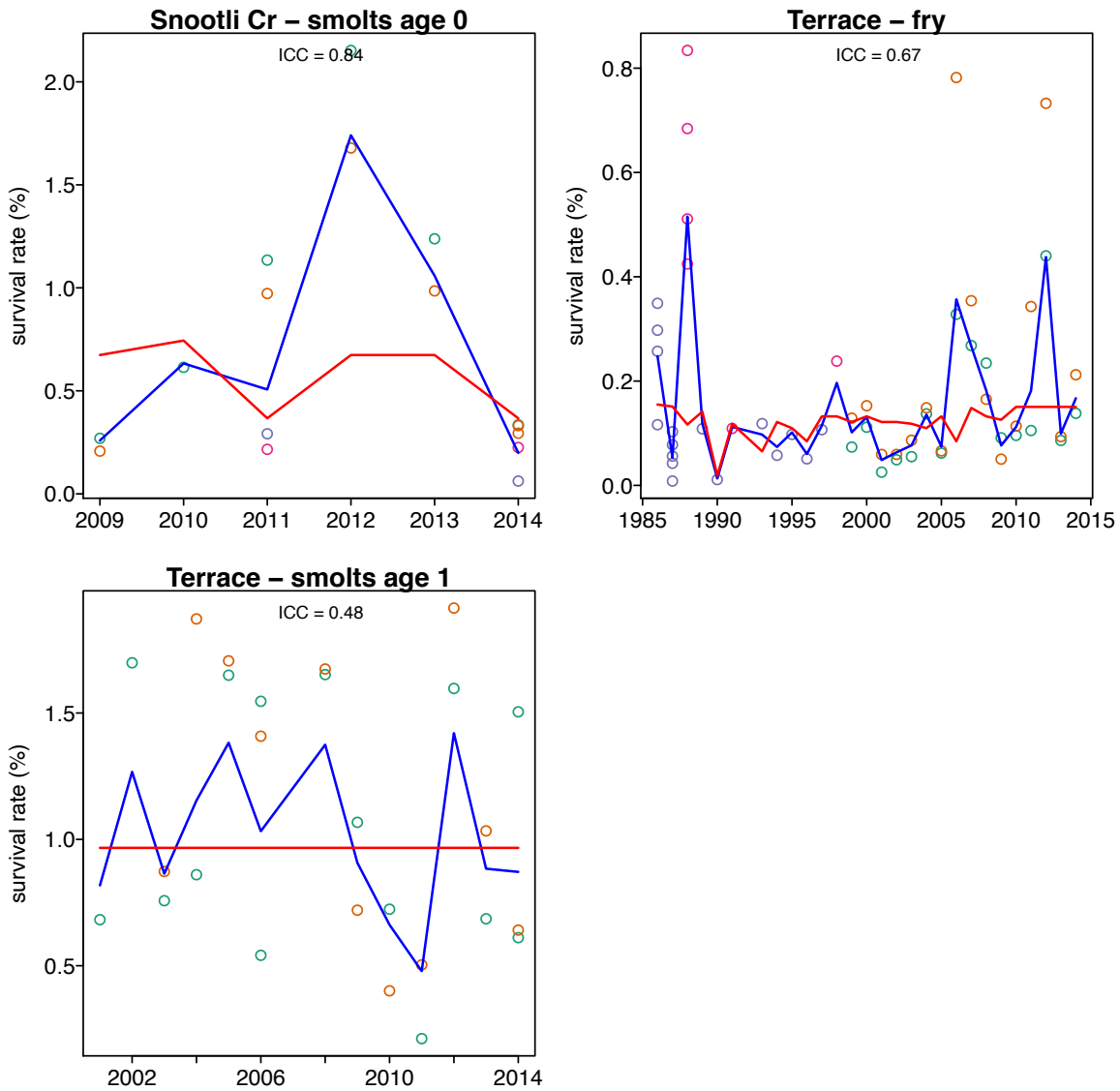
Figure CH.21. Top model fits for Northern BC hatcheries’ average Chinook survival over time, accounting for all predictors (e.g. weight, day, year, stock, and release site) with (blue) and without (red) random year effects. Different colors indicate different combinations of stocks and release sites for each hatchery with green indicating the most frequent stock released and release site.
