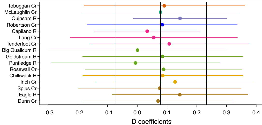
Figure A.15. Multi-hatchery Coho survival model coefficient estimates for initial model fits including hatchery deviations for river migration distance ( M ) and linear terms for Day ( D ) at-release. The circles indicate hatchery specific estimates along with 95% CIs, while the vertical lines indicate the average effect (thick black line) across all hatcheries with 95% CIs (thin black lines).
