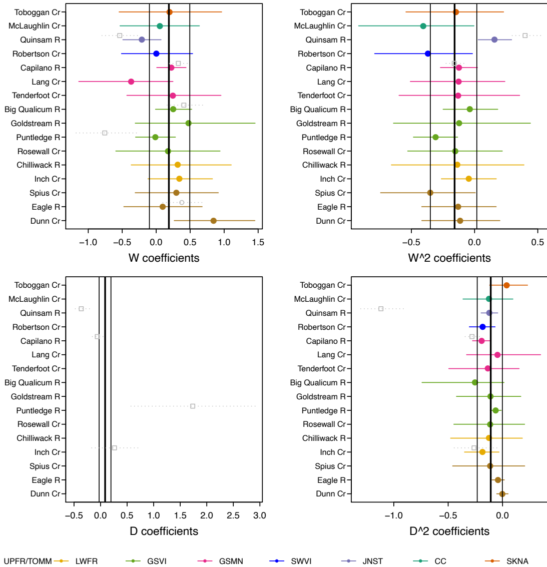
Figure CO. 29. Coho multi-hatchery survival model coefficient estimates for linear and quadratic terms for Weight ( W , W^2 ) and Day ( D , D^2 ) at-release. The circles indicate hatchery specific mean posterior estimates along with 95% credible intervals, while the vertical lines indicate the mean posterior for the average effect across all hatcheries (thick black line) with 95% credible intervals for the posterior distribution (thin black lines). Single-hatchery estimates and 95% CIs are shown in grey for fry (○) or yearling smolt (□) life-stage specific models.
