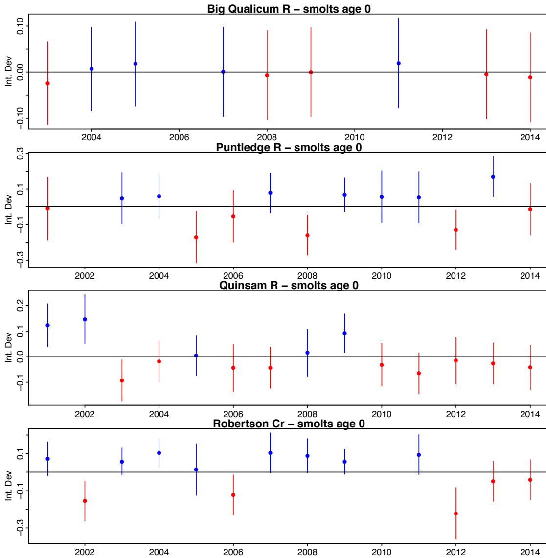
Figure CH.27. The ocean entry year-effect deviation in average Chinook age of returns (i.e., \Delta_t ) for each hatchery and life-stage model. Negative (red) values indicate a year effect below the average and positive (blue) values indicate a year effect above the average.
