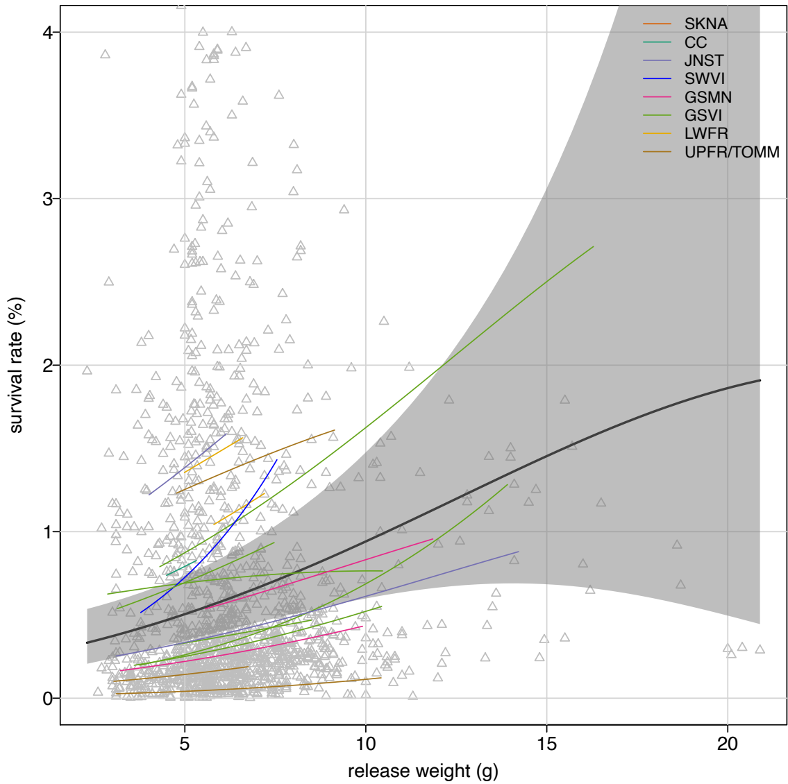
Figure A.16. Hatchery average Chinook survival and hatchery-specific survival responses for the central 95% distribution of observed weights-at-release for each hatchery for models fit with only sub-yearling smolt data . The black line (MLE) and shaded areas (95% CI) indicate the average weight effect on survival across all hatcheries, while coloured lines show hatchery-specific estimates (MLEs). Note observations with survival rates greater than 4% are not shown.
