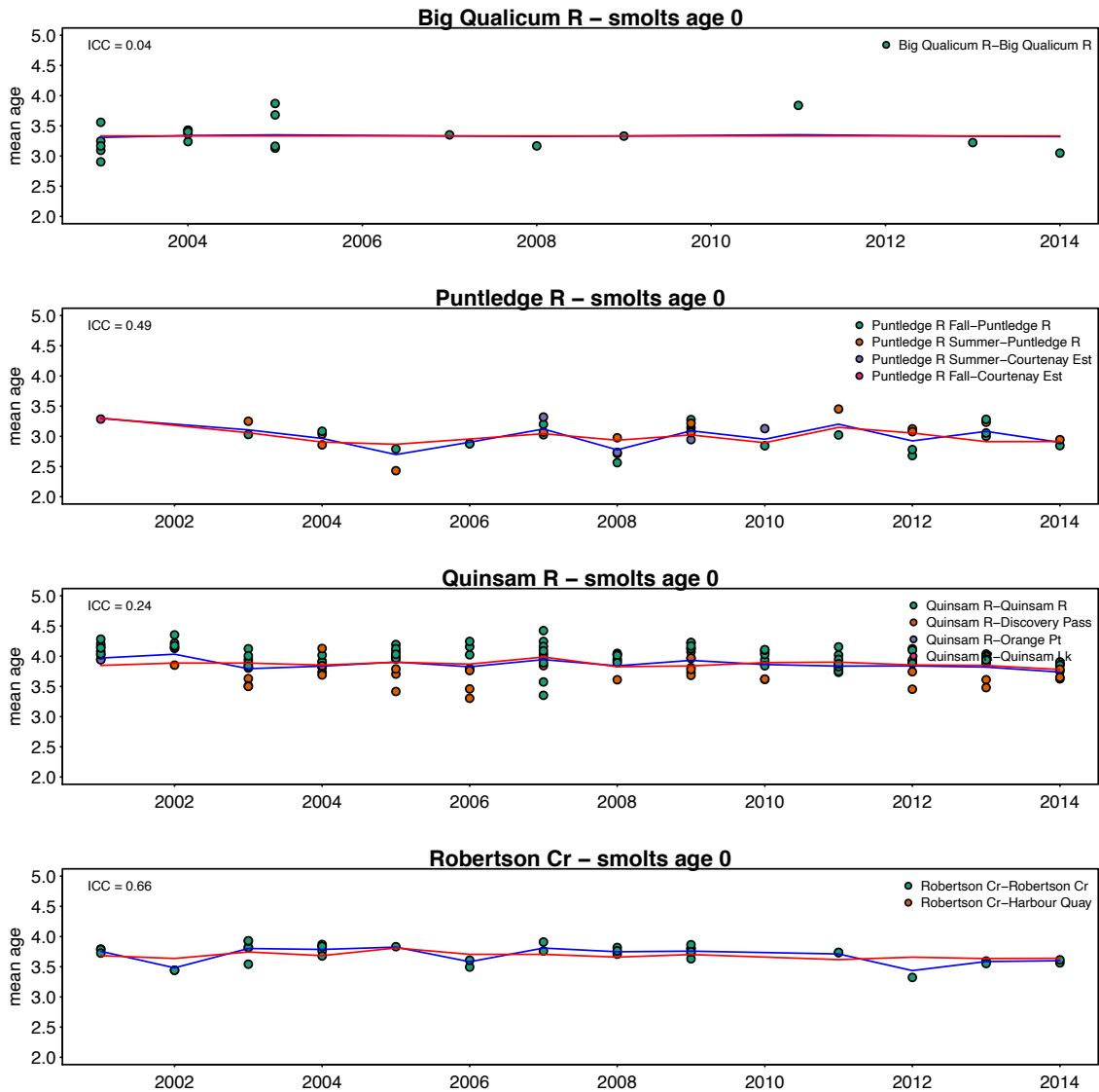
Figure CH.26. Top model fits for BC hatcheries' mean Chinook return age over time, accounting for all predictors (e.g. weight, proportion of females, stock and release site) with (blue) and without (red) random year effects.
