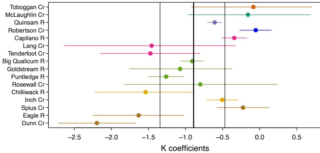
Figure CO.38. Coefficient estimates for multi-hatchery Coho survival models fit with Harbour Seal (H) and Killer Whale (K) covariates. The circles indicate hatchery specific mean posterior estimates along with 95% credible intervals, while the vertical lines indicate the mean posterior for the average effect across all hatcheries (thick black line) with 95% credible intervals (thin black lines).
