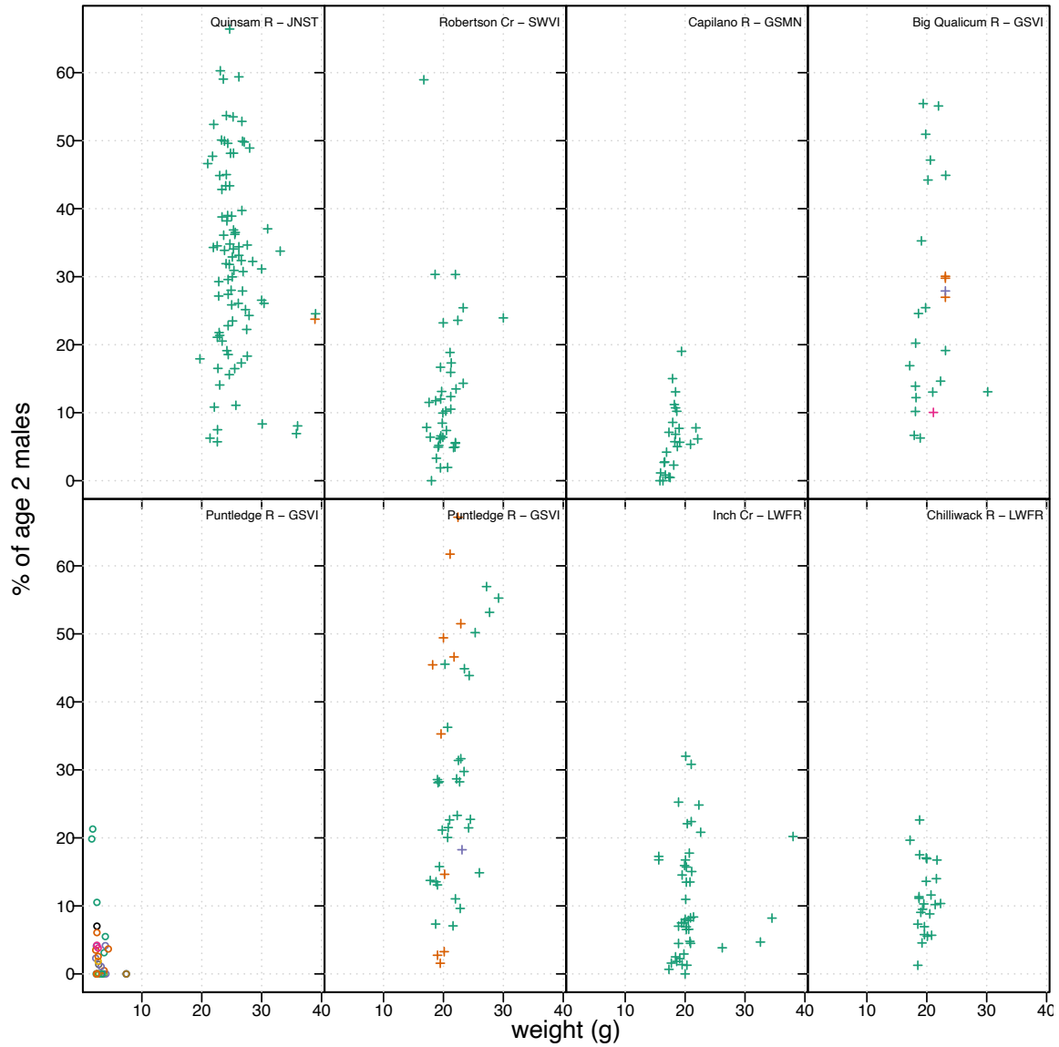
Figure CO.9. Proportion of age-2 males in male returns by weight-at-release for fry (○) and yearling (+) CWT Coho hatchery releases included in return age model fitting . Different colors indicate different combinations of stock and release sites for each hatchery with green indicating the most frequent stock released and release site.
