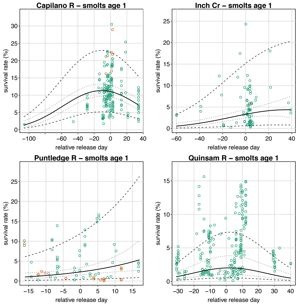
Figure CO.17. Mean survival (solid line) for Coho at release days for hatchery and life-stage specific model fits. The 95% CIs are shown for fixed effects only (dotted lines) and for both fixed and random year effects (dashed lines). The zero day indicates the mean release date for a hatchery, while different colours indicate different combinations of stocks and release sites. Hatcheries without Day effects in top models are not shown. Hatcheries without Day effects in top models are not shown.
