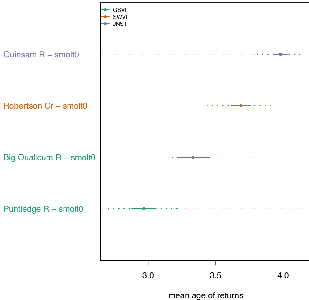
Figure CH.23. Mean Chinook return ages and 95% confidence intervals accounting for uncertainty in both fixed and random effects for top model fits for each hatchery. Solid lines indicate uncertainty due to fixed effects, while the dotted lines indicate uncertainty from both fixed and random year effects. The mean ages reflect estimated survival for the average values of covariates.
