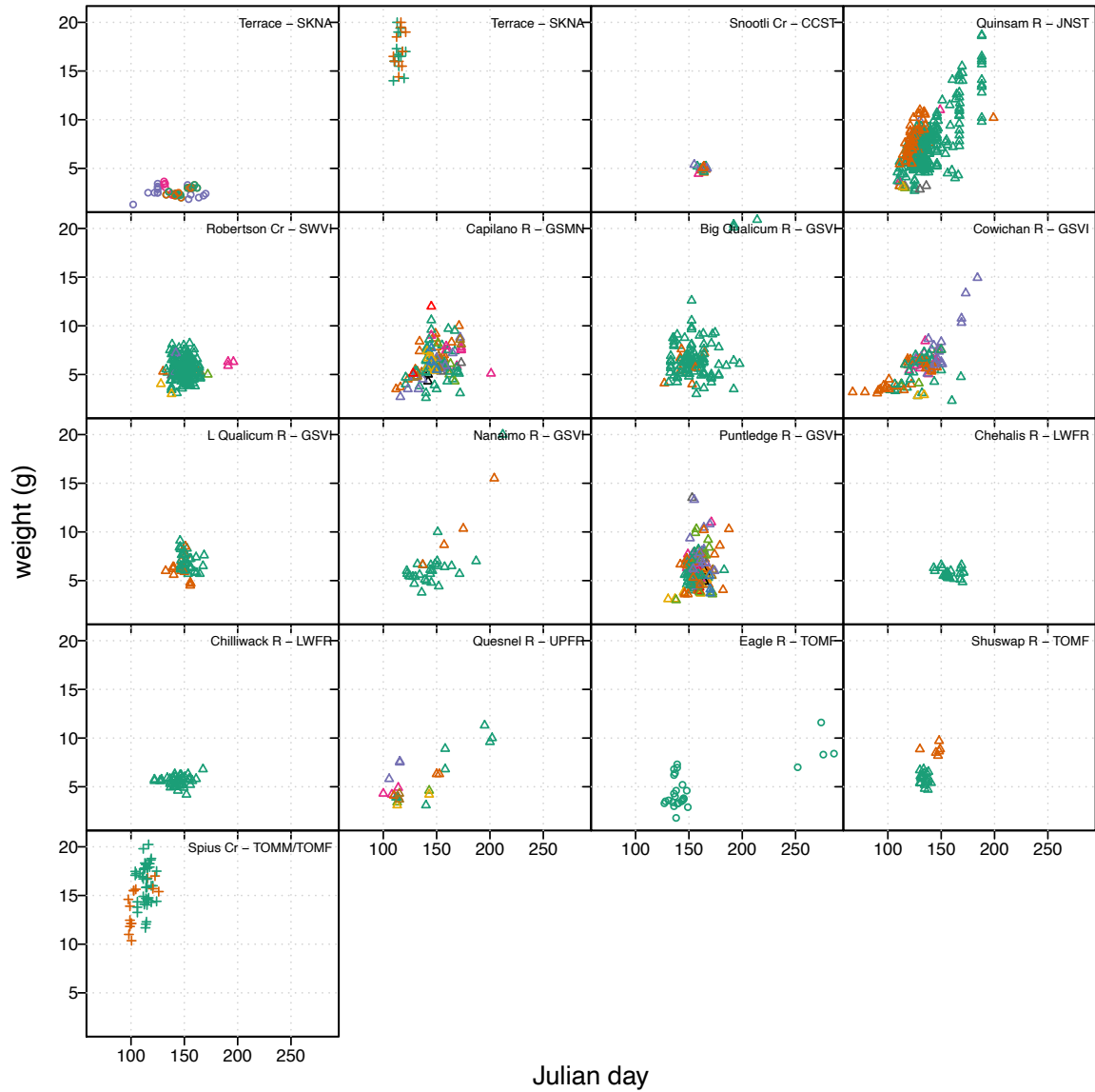
Figure CH.6. Weight-at-release by Julian day for fry (○), smolt (△), and yearling (+) CWT Chinook hatchery releases included in survival model fitting. Different colors indicate different combinations of stock and release sites for each hatchery with green indicating the most frequent stock released and release site.
