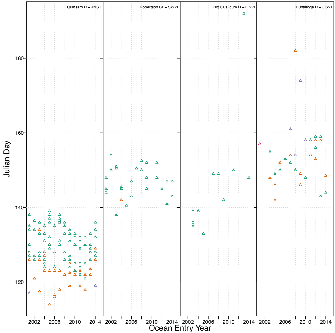
Figure CH.14. Julian day-at-release by ocean entry year for smolt ( \triangle ) CWT Chinook hatchery releases included in return age model fitting . Different colors indicate different combinations of stock and release sites for each hatchery with green indicating the most frequent stock released and release site.
