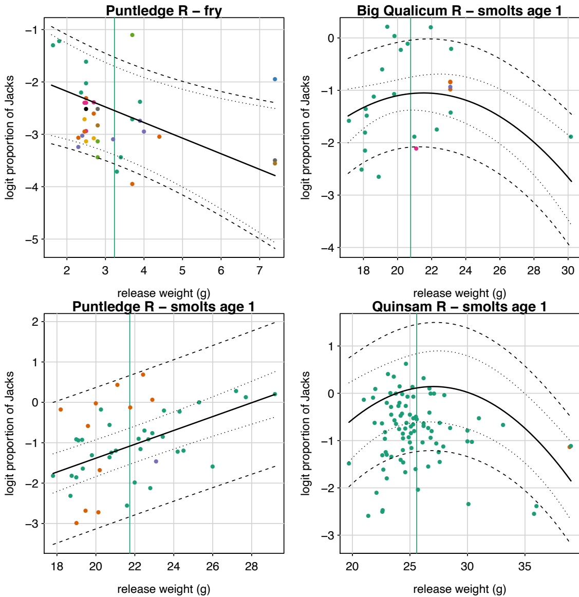
Figure A.12. Mean logit proportion of age age-2 male returns (solid line) for Coho at different release weights for hatchery and life-stage specific model fits. The 95% CIs are shown for fixed effects only (dotted lines) and for both fixed and random year effects (dashed lines). Different colours indicate different stocks released and the solid green vertical line indicates the mean weight-at-release.
