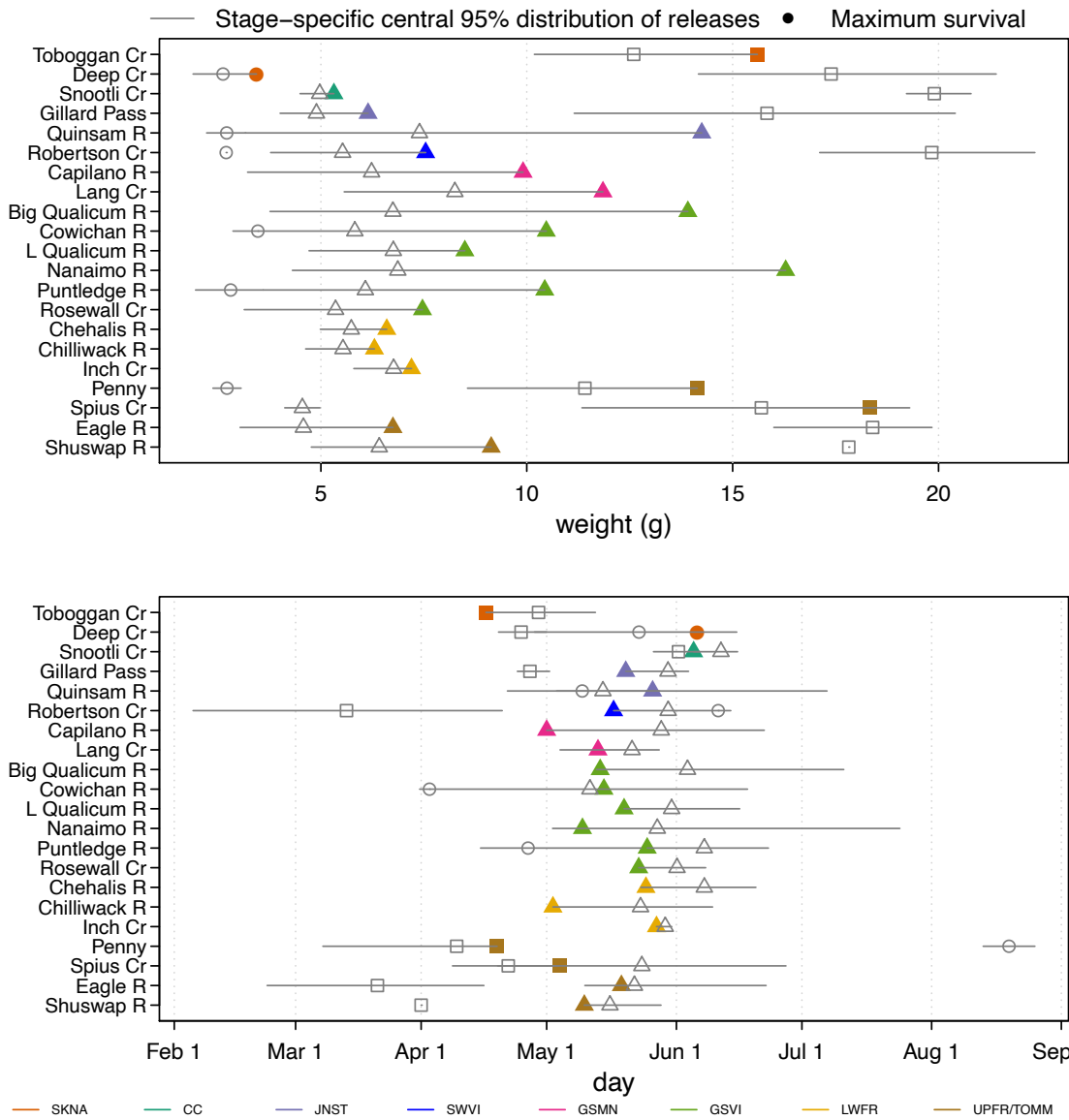
Figure CH.33. Optimal weights (top) and days-at-release (bottom) for maximum Chinook survival for multi-hatchery model posterior means. For each hatchery, the horizontal lines indicate the central 95% distribution of release weights or days for each life-stage (some of which overlap) with means for fry (○), sub-yearling (△) and yearling smolts (□). The coloured circle indicates the release weight or day within the central 95% distribution of observations (grey line) that is expected to maximize survival for the life-stage most commonly released at each hatchery.
