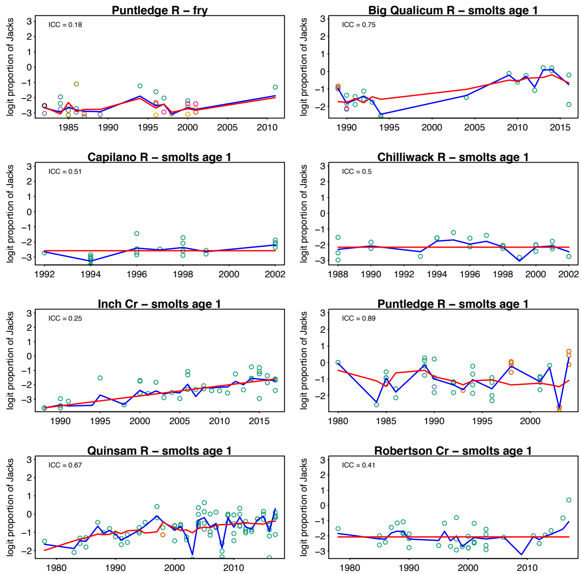
Figure A.13. Top model fits for BC hatcheries' logit proportion of age-2 males in Coho returns over time, accounting for all predictors (e.g. weight, proportion of females, stock and release site) with (blue) and without (red) random year effects.
