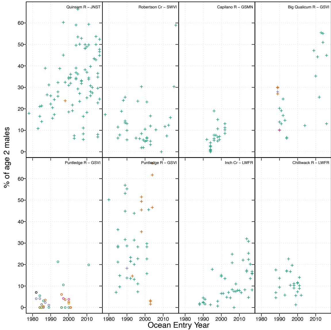
Figure CO.11. Proportion of age-2 males in male returns by ocean entry year for fry (O) and yearling (+) CWT Coho hatchery releases included in return age model fitting . Different colors indicate different combinations of stock and release sites for each hatchery with green indicating the most frequent stock released and release site.
