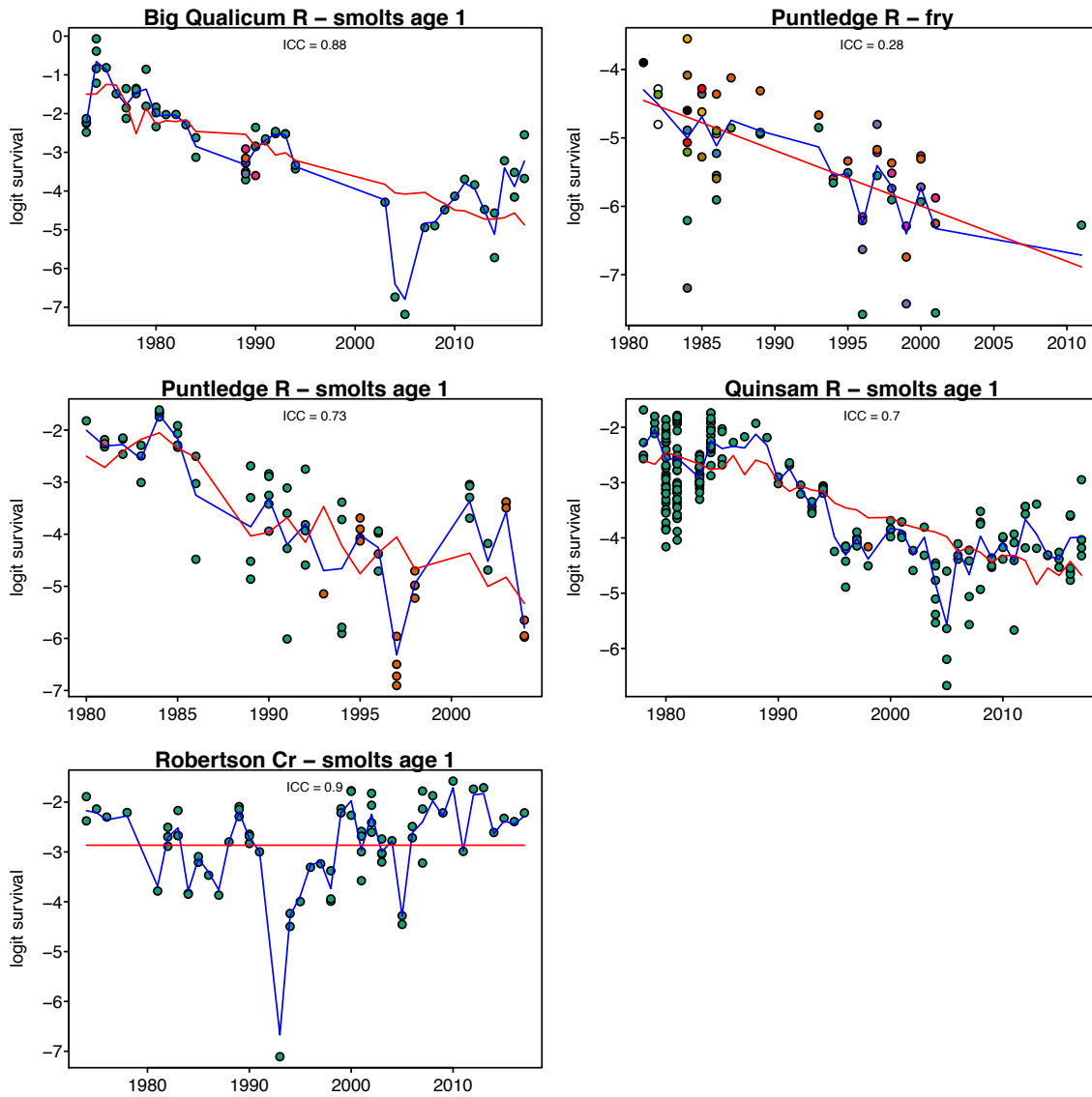
Figure A.10. Top model fits for Vancouver Island hatcheries' average Coho logit survival over time, accounting for all predictors (e.g. weight, day, year, stock, and release site) with (blue) and without (red) random year effects.
