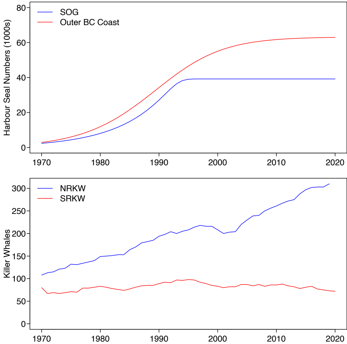
Figure A.20. Top: Harbour Seal numbers for the Strait of Georgia (SOG) and outer BC coast for 1970-2020 based on models from Olesiuk et al. 2010. Bottom: Annual numbers of Northern Resident Killer Whales (NRKW, Chasco et al. 2017, Towers et al. 2020) and Southern Resident Killer Whales (SRKW, Centre of Whale Research Data).
