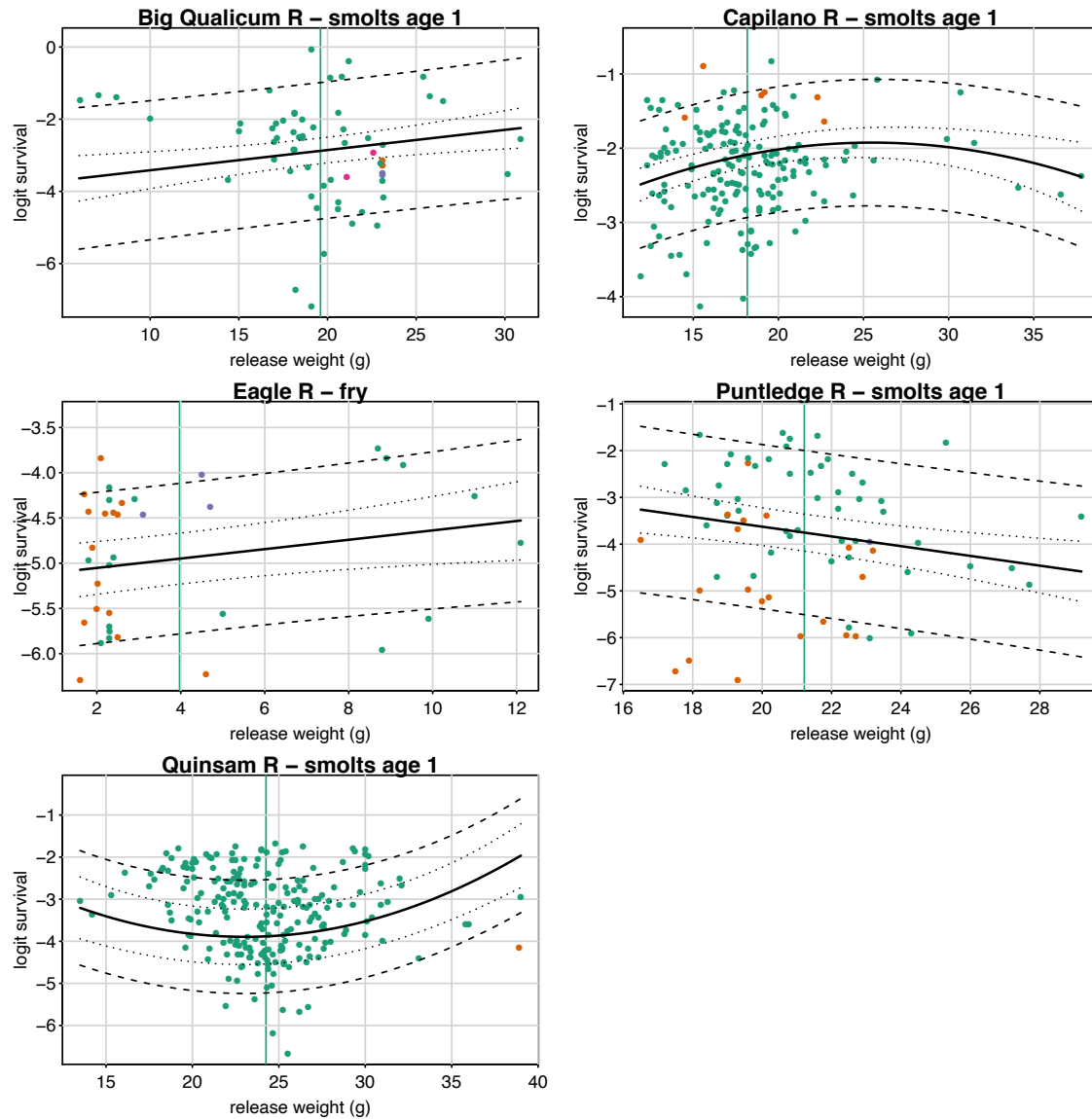
Figure A.7. Mean logit survival (solid line) for Coho at different release weights for hatchery and life-stage specific model fits. The 95% CIs are shown for fixed effects only (dotted lines) and for both fixed and random year effects (dashed lines). Different colours indicate different stocks released and the solid green vertical line indicates the mean weight-at-release.
